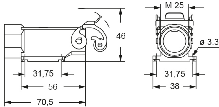
Catalogue drawings
