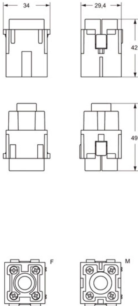
Catalogue drawings
